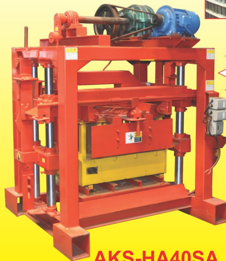
Hollow Brick 390 x 190 x 200 mm
